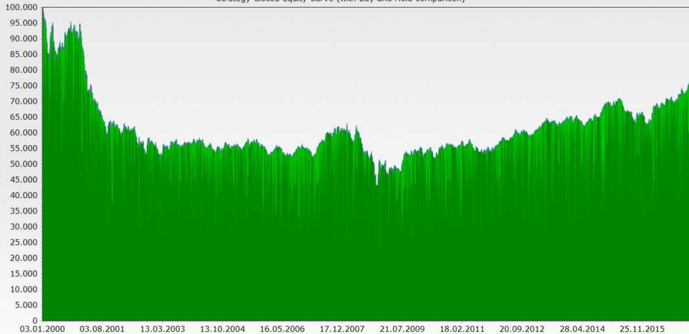
Strategy Closed Equity Curve (with Buy and Hold comparison)
